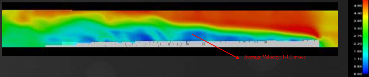
Velocity Profile – 4.5 m/sec – With Berm
