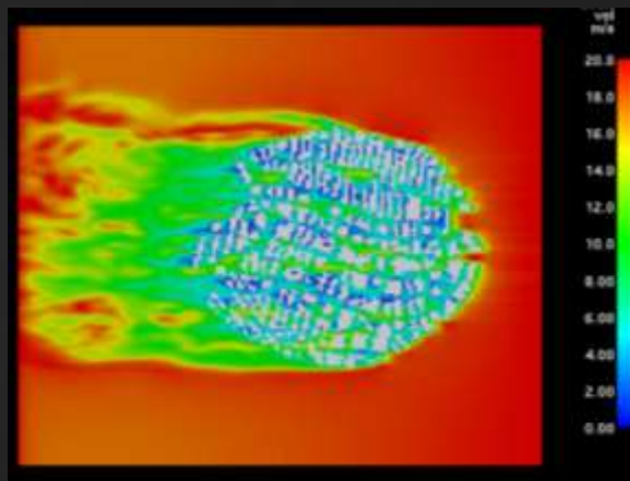
Velocity Profile – 20 m/sec
