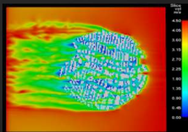
Velocity Profile – 4.5 m/sec
