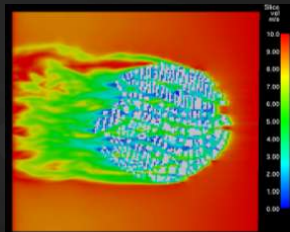
Velocity Profile – 10 m/sec
