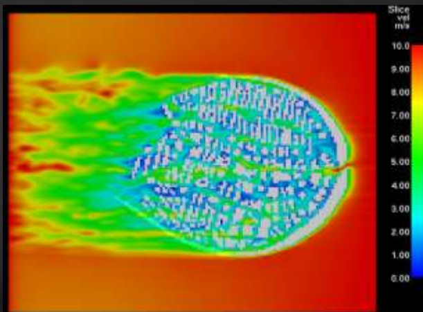
Velocity Profile – 10 m/sec
