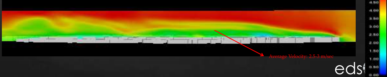
Velocity Profile – 4.5 m/sec – Without Berm
